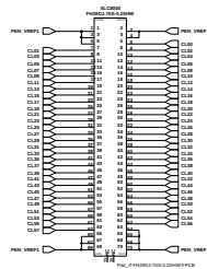
70pin S-PEN Connector
