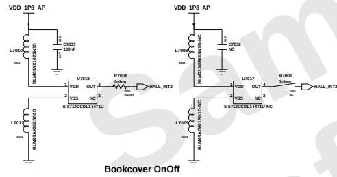
Hall Sensor SEIKO
