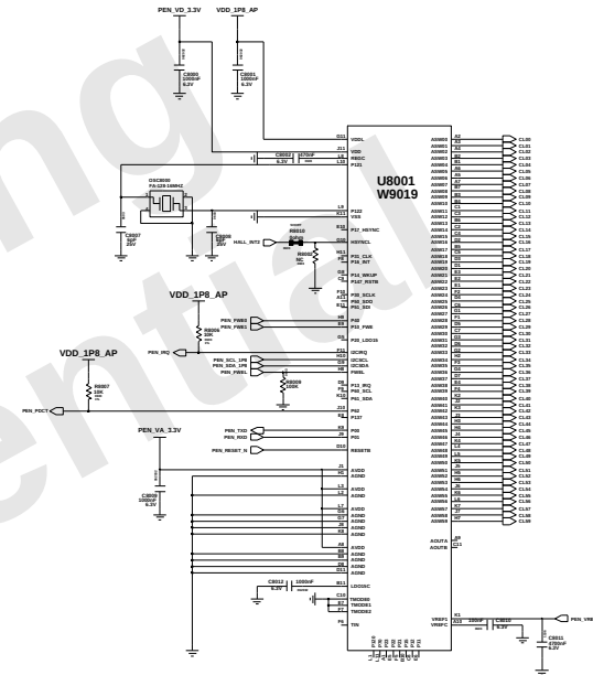
S_PEN Control IC
